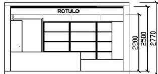
ALZADO PRINCIPAL
